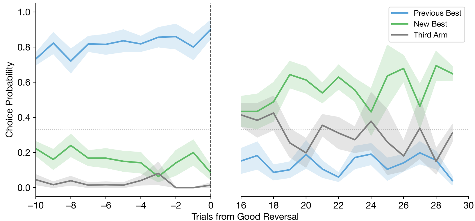
Good Reversal-Aligned Choices (mean \pm se across subjects | n=5 subjects, n=50 reversals) (Skipping first 15 trials post-reversal)
